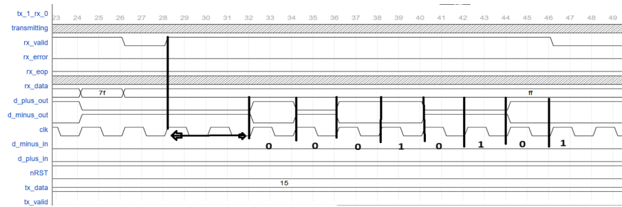
Figure 7: Transmitting 8'b00010101 Byte Waveform
